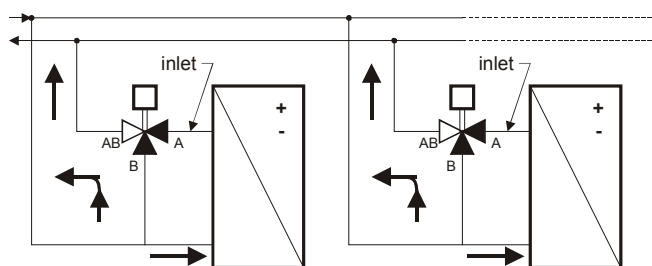
Fig. 2. Three-way valve operation
